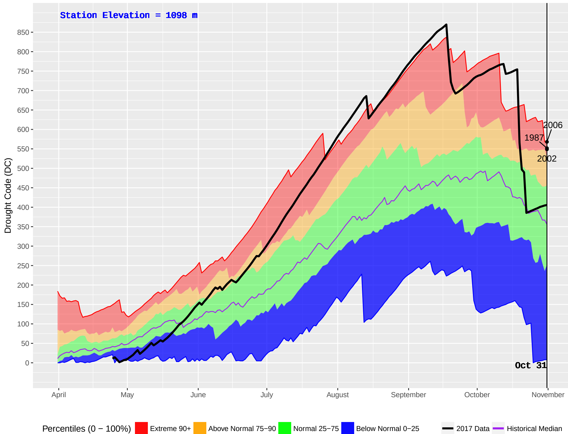
GOATFELL (401) : Historical (1986–2016) and Current (2017) Noon Drought Code (DC)
