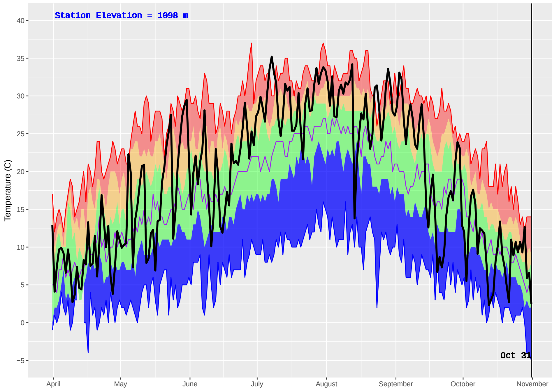
GOATFELL (401) : Historical (1986–2016) and Current (2017) Noon Temperature
