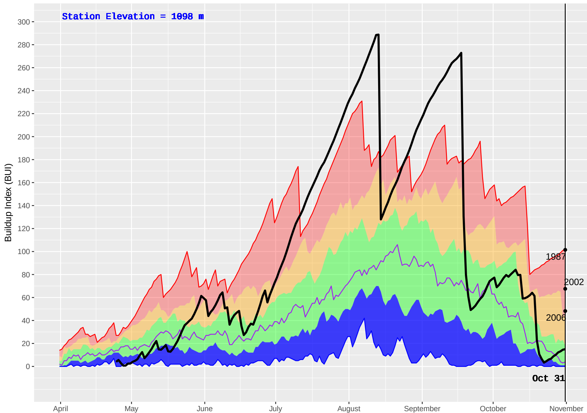
GOATFELL (401) : Historical (1986–2016) and Current (2017) Noon Buildup Index (BUI)
